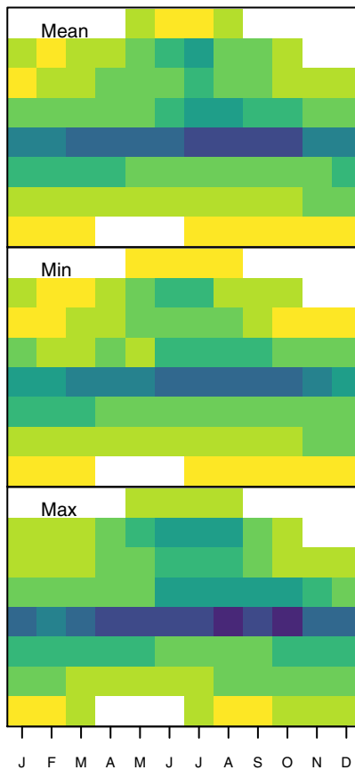
(b) LAI Reference Ensemble (N = 2 )
