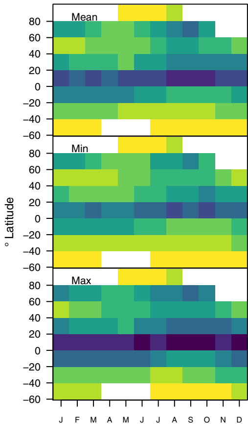
(a) LAI Model Ensemble (N = 6 )
