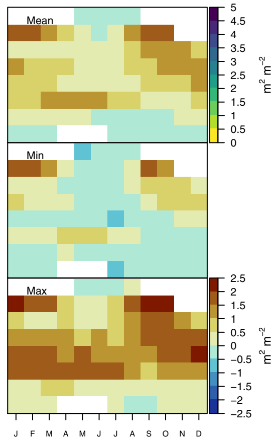
(c) LAI Mean Ensemble Bias (N = 12 )
