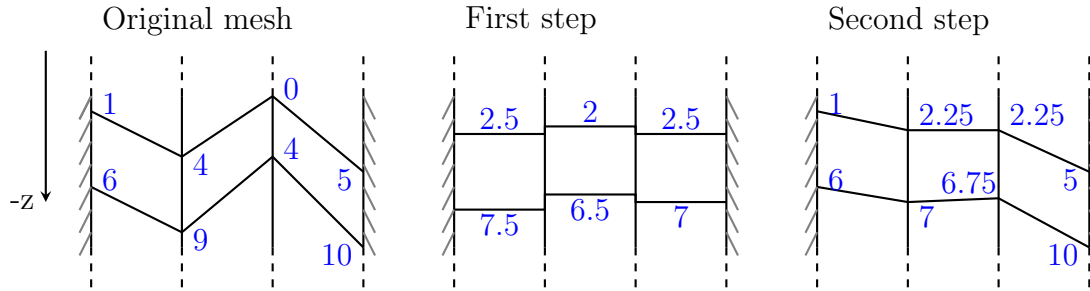
Figure 5. Illustration of the horizontal smoothing algorithm on a 2D x - z mesh. First, for each element, the upper and lower nodal values of the vertical coordinate z are set to their mean value, then z is projected onto a continuous field. The numbers refer to the depth of the mesh levels.
